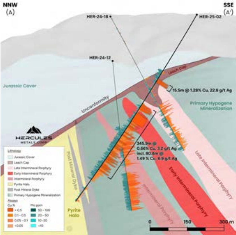
(L-to-R): Photo 1: HER-25-02 cross section; Photo 2: Examples of hypogene enrichment at Leviathan. (A). Hypogene chalcocite veins and disseminations. (B). Covellite (blue, white circle) intergrown and encompassed within thick chalcocite veins and disseminations. (C). Covellite (blue, white circle), rimmed by bornite (purple), complexly intergrown with pyrite, indicative of high-sulfidation fluid conditions (hypogene enrichment). (D). Covellite (blue) and bornite (purple) veins crosscut by later chalcopyrite veins. HQ size core.
